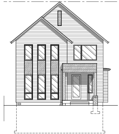
FRONT ELEVATION (WEST)
