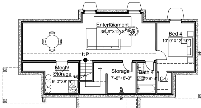
BASEMENT
