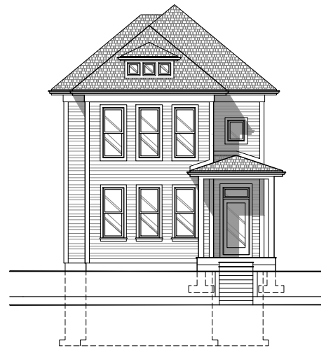
FRONT ELEVATION (WEST)
