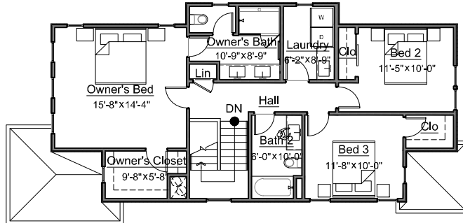
SECOND FLOOR
