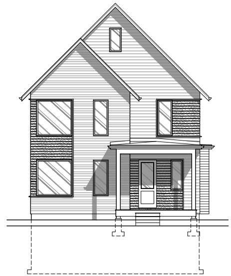
FRONT ELEVATION (WEST)
